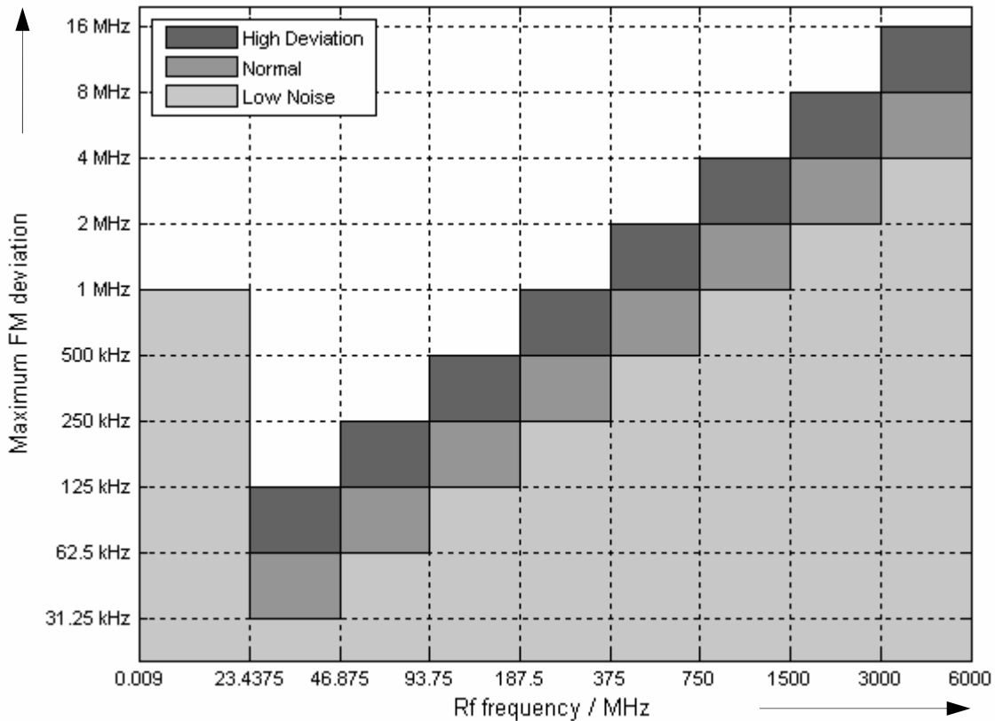
FM deviation versus frequency and operating mode
