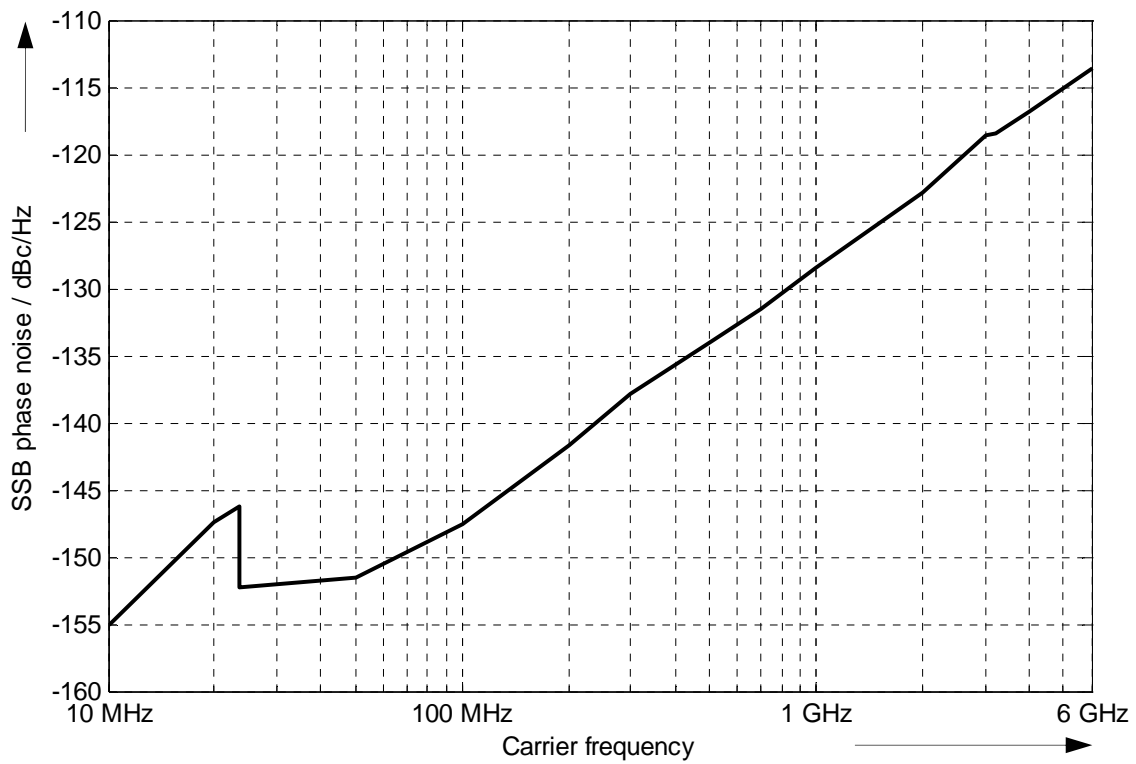
Measured SSB phase noise at 20 kHz offset versus frequency with internal OCXO (R&S®SMB-B1 option)
