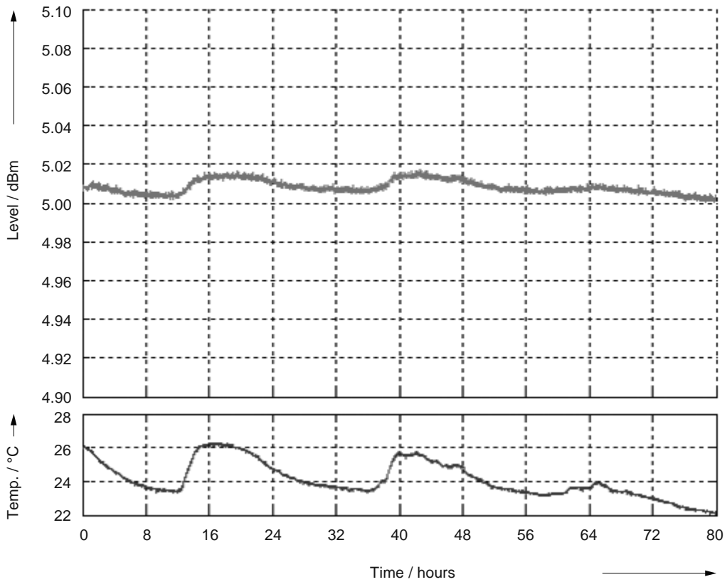
Measured level repeatability at 3 GHz, 5 dBm, ALC ON
