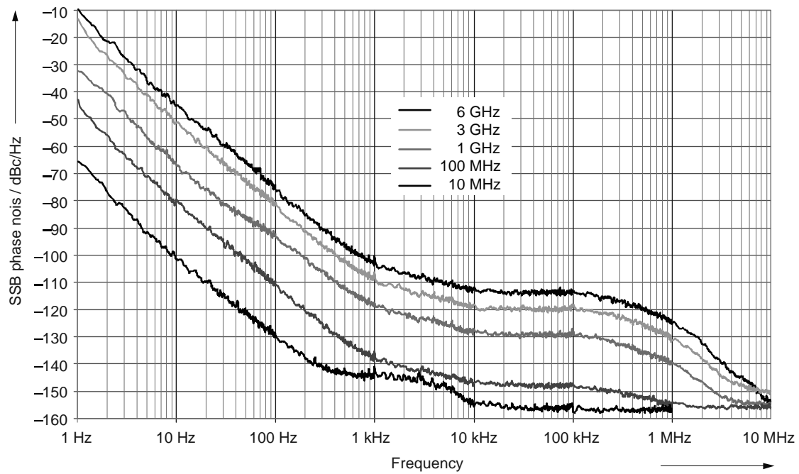
Measured SSB phase noise
