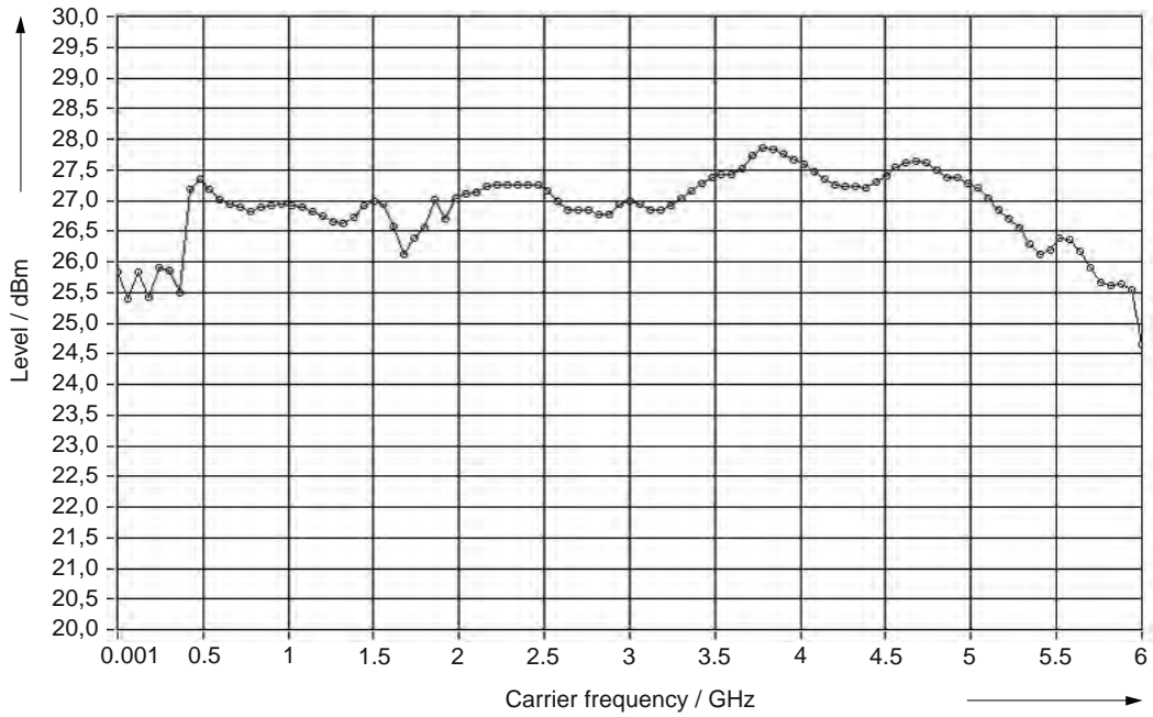
Measured maximum output power versus frequency
