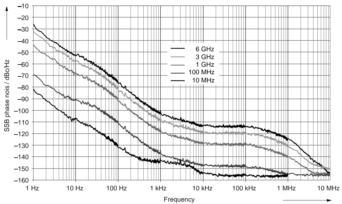
Measured SSB phase noise with internal OCXO (R&S ® SMB-B1 option)
