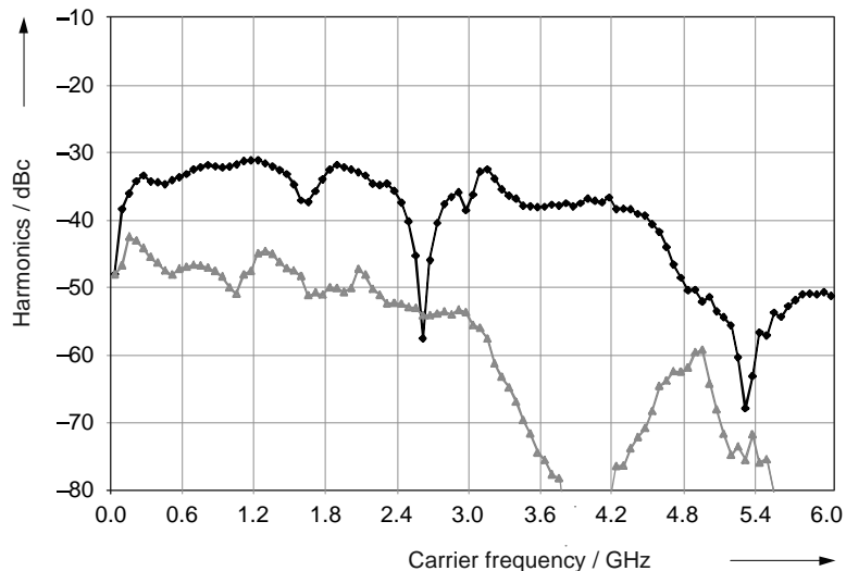
Measured harmonics at +18 dBm versus frequency
